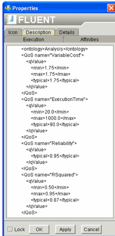
Figure 4.5 QoS description
