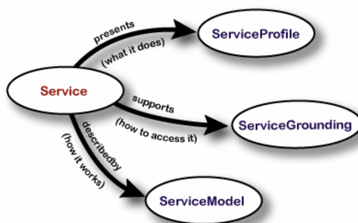
Figure 2.1 OWL-S description [21]
